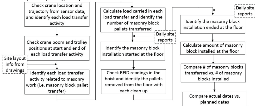
Figure 6: Data fusion approach for identifying masonry work progress at a floor
