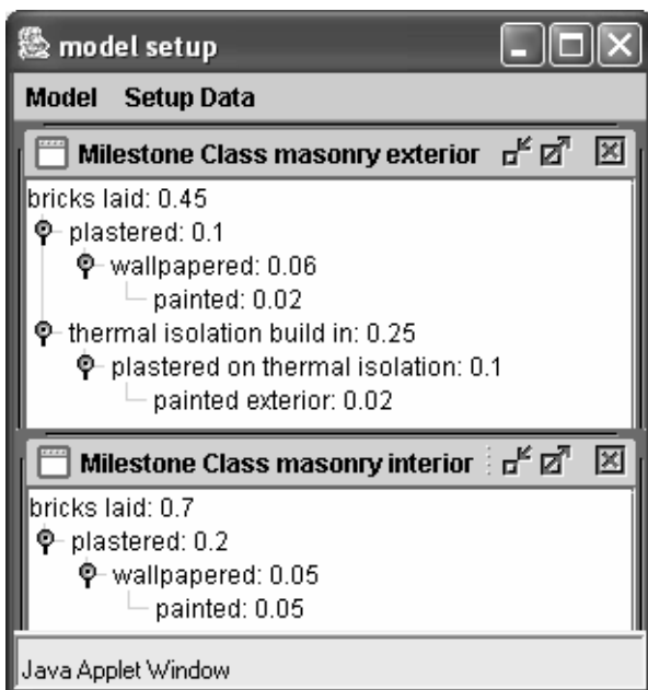
Figure 10. Weighted states
