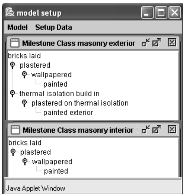
Figure 1. Milestone classes
