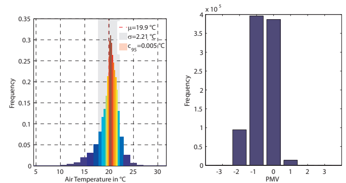
a) Room air temperature. b) Room PMV.
