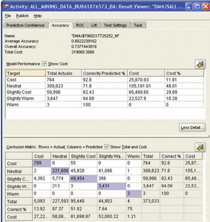
Figure 6. Model accuracy and the confusion matrix.
