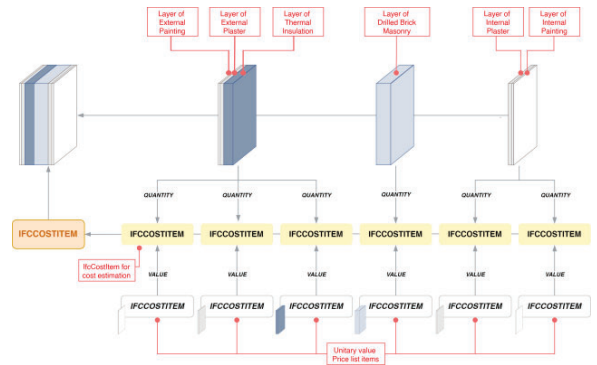
Figure 7 Example wall consists of six layers
