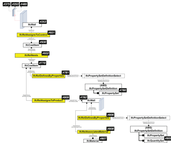
Figure 13 Relationships activated by IfcCostItem with relative identification number
