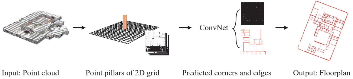
Figure 3: Pipeline of the learning for 2D reconstruction.
