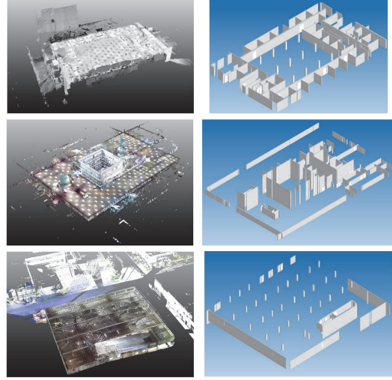
Figure 10: Examples of 3D reconstruction by FLKPP.
