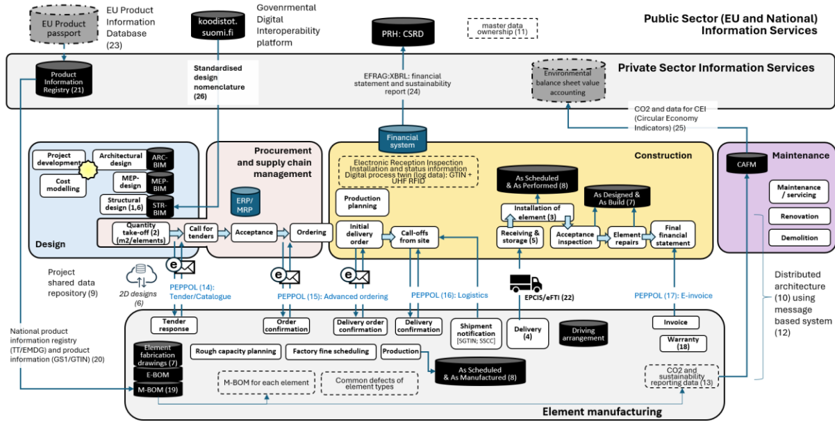
Figure 2. The data repositories of the element supply chain, the proposed standards in the national model, the data flows, as well as the key process steps in the design, procurement, manufacturing, delivery, and installation of elements.
